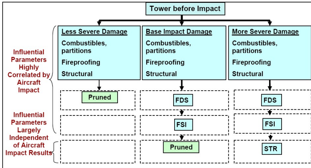
Figure 9-3. Pruned analysis tree for influential parameter effects.
